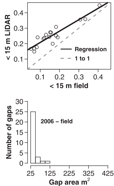
Figure 5 Validation of remote measurements in an old-growth tropical rain forest. The proportion of canopy height measurements < 15.00 m within 18 0.5 ha plots is highly correlated using field measurements and light detection and ranging (LiDAR) remote sensing. Canopy gaps > 125 m 2 were not represented in plots, but simulations suggest this is an artifact of the smaller area sampled, because larger gaps are rare within the old-growth landscape and the MLE of the power-law exponent is marginally significantly different between plots and the old-growth landscape (one-tailed P = 0.069 , based on 2000 nonparametric bootstrap samples).
